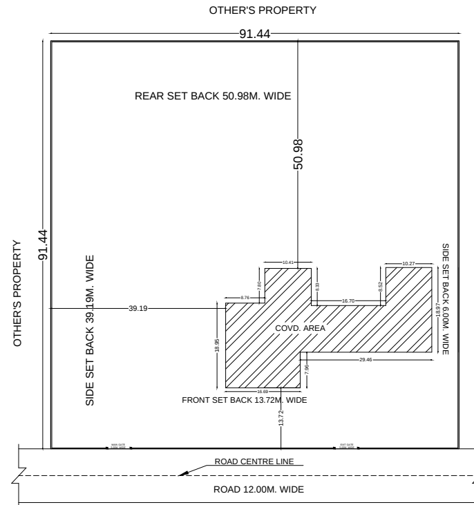
FIRE FIGHTING/SITE PLAN
